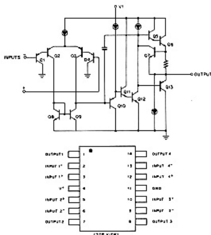
Fig.7 NJM2902N (PLL UNIT Q25) K TYPE ONLY
