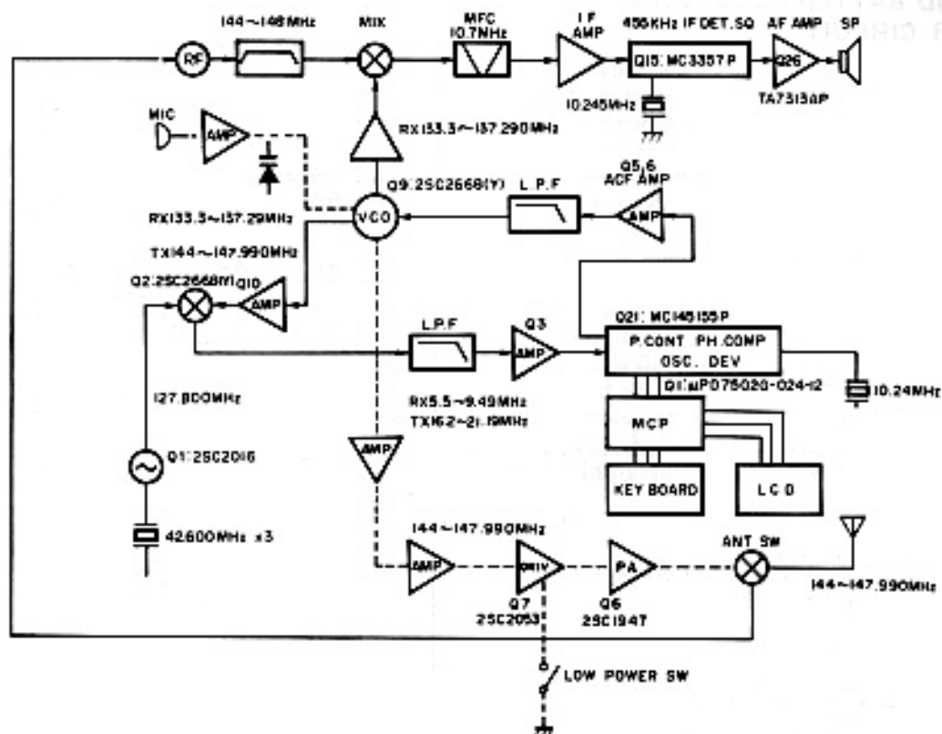
Fig.13 Frequency configuration
