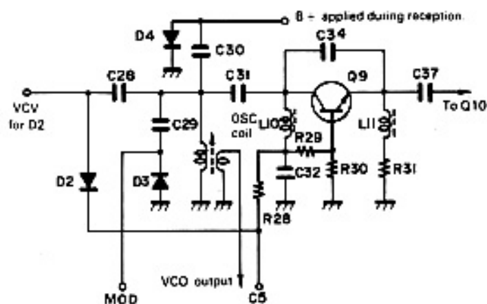
Fig.4 VCO circuit
