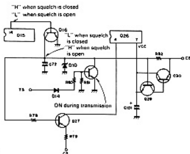
Fig.3 Squelch circuit
