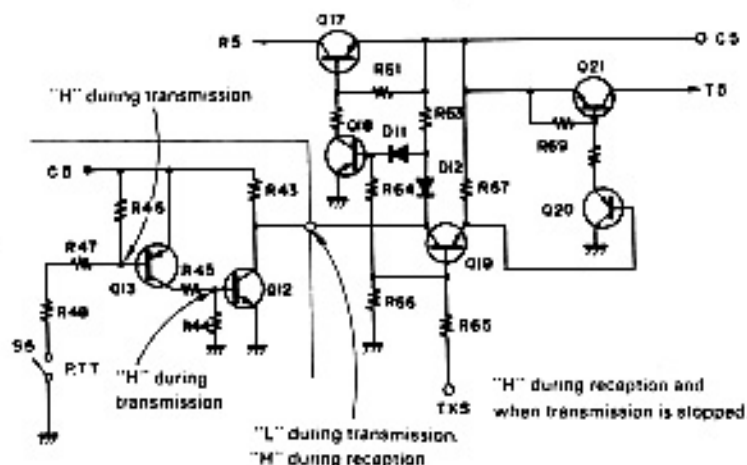
Fig.8 Transmission (T5) and Reception (R5) Voltage Generation circuit (TX,RX UNIT)
