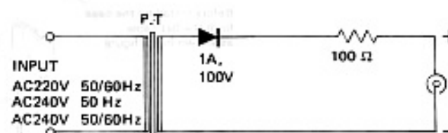
Fig. 12 W09-0317-05, W09-0318-05, W09-0319-05 Schematic diagram
